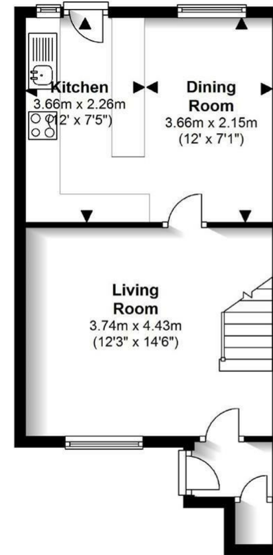
Ground Floor Approx. 35.4 sq. metres (381.0 sq. feet)
